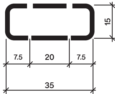
2 Lochreihen
